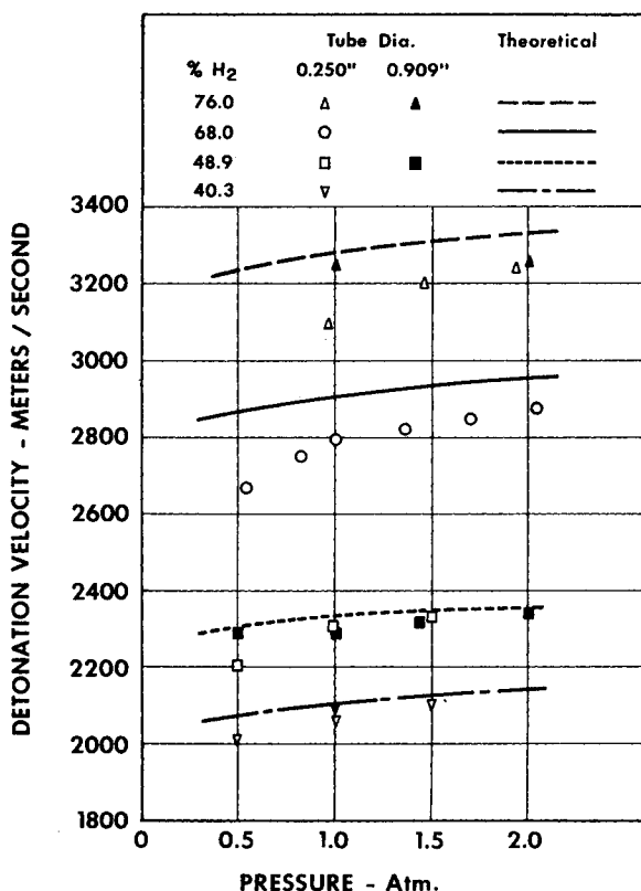
Fig. 4. The effect of initial pressure on detonation velocity at 298°K.
