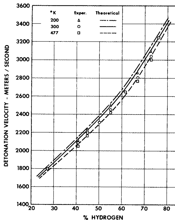
Fig. 5. Detonation velocities at several initial temperatures and 1 atm.
